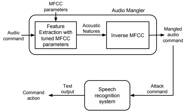
Figure 2: Attack outline.
