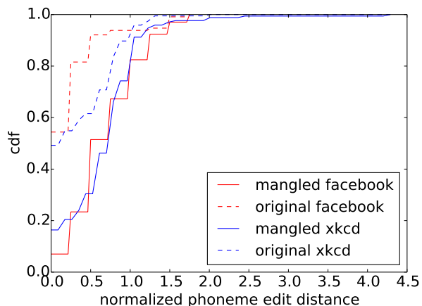
Figure 4: Cumulative distribution of phoneme edit distances, for both the original and mangled audio, for the commands that open Facebook and the xkcd website.
