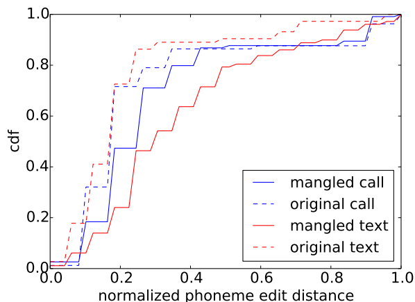
Figure 5: Cumulative distribution of phoneme edit distances, for both the original and mangled audio, for the commands that send an SMS message (“original/mangled text”) and place a call (“original/mangled call”).
