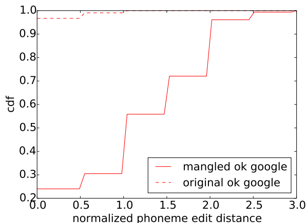
Figure 3: Cumulative distribution of phoneme edit distances, for both the original and mangled audio, for the “Ok Google” command.
